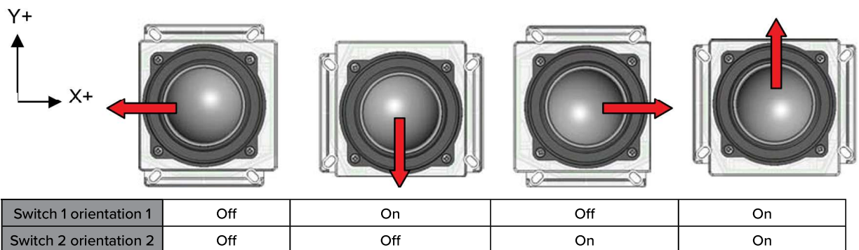
Figure.1 Mounting orientations
